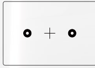
Mercedes-Benz - LDW Calibration Board
